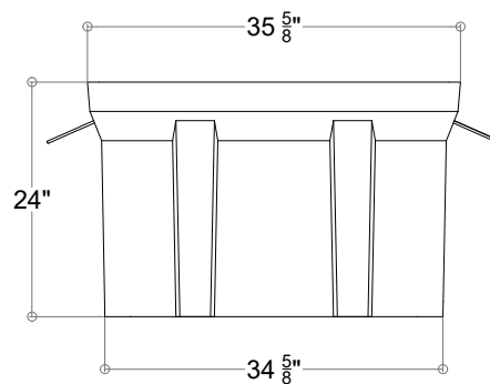
BOX FRONT VIEW
