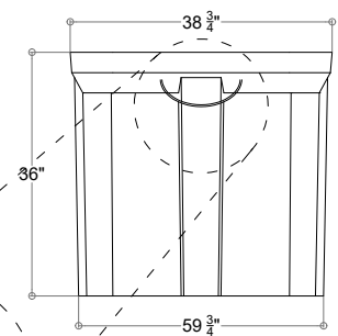
BOX SIDE VIEW
