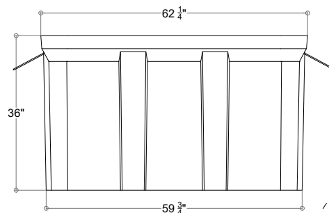
BOX FRONT VIEW
