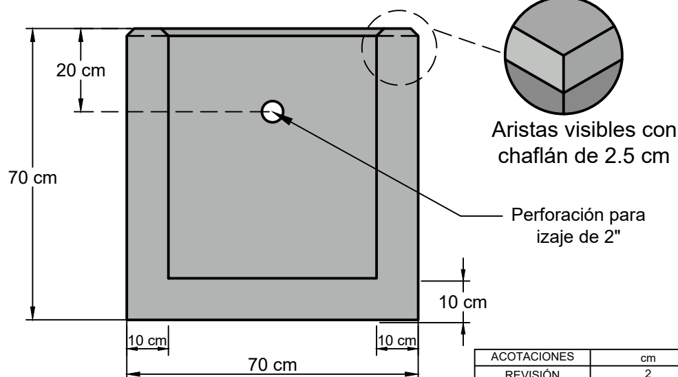
Vista Frontal
