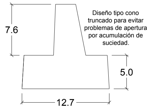
Detalle Brocal
