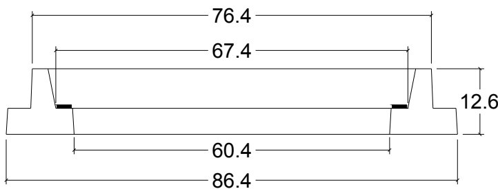
Vista Lateral Brocal
