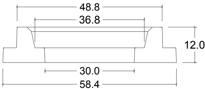
Vista Lateral brocal
